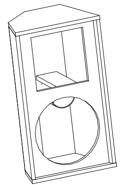
F122A(+N) general dims Material 15mm Birch Plywood
