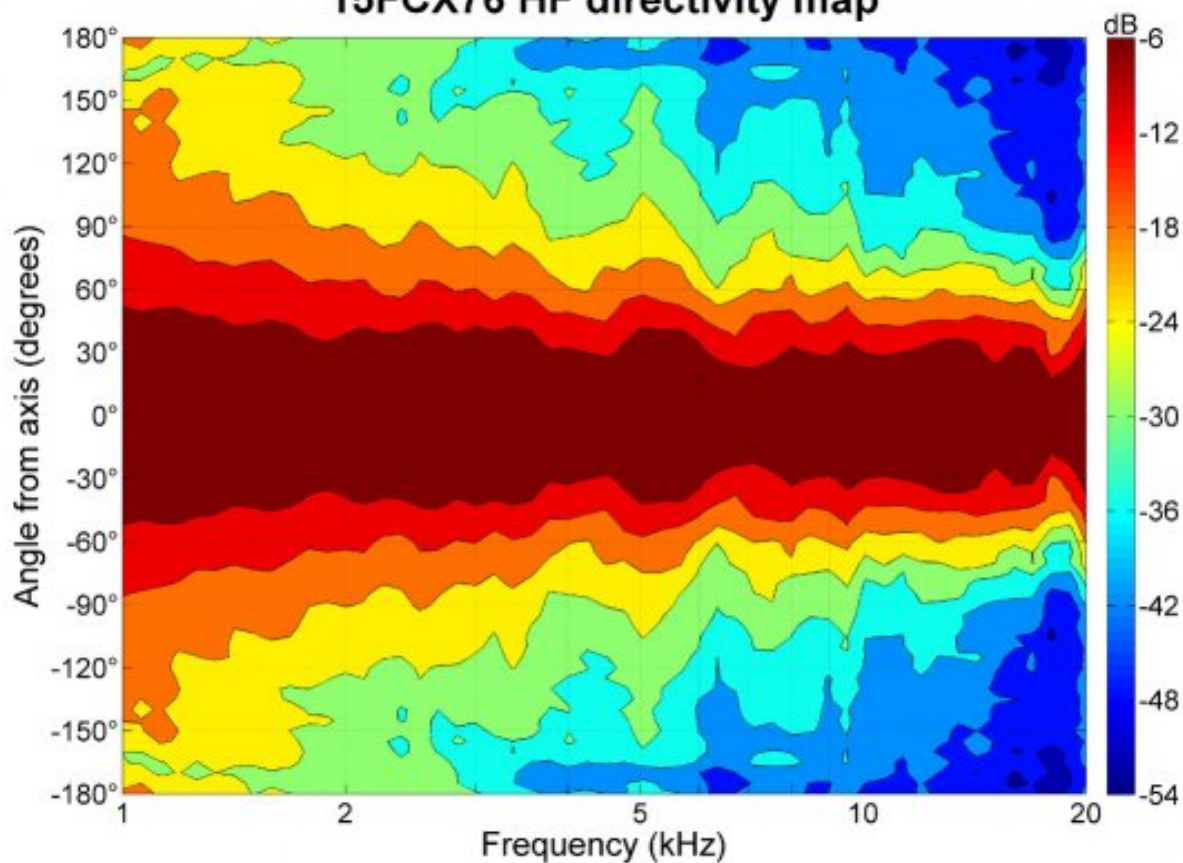
15FCX76 HF directivity map
