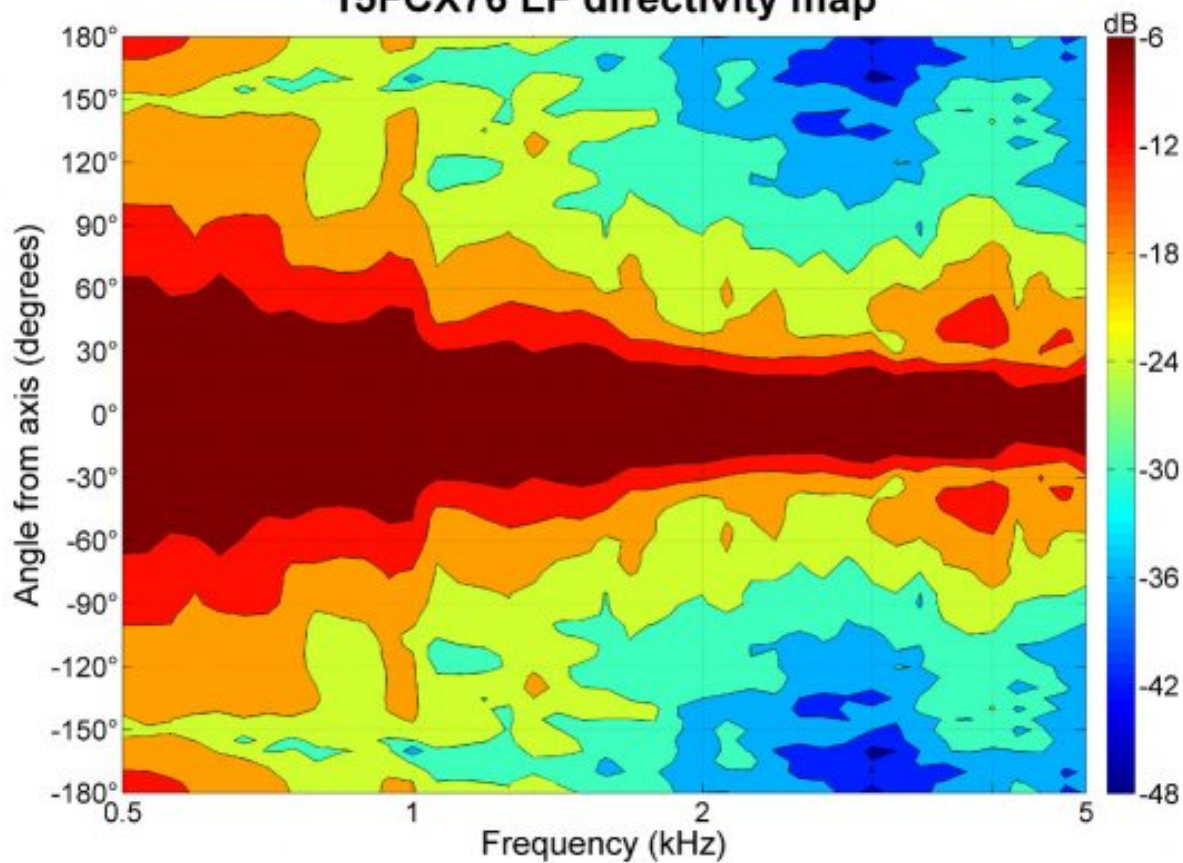
15FCX76 LF directivity map
