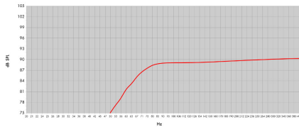
Frequency Response [1W/1m]
